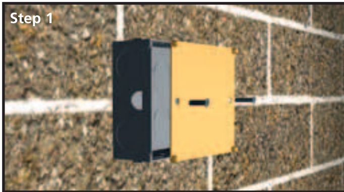
Step 1 Fit Sockitz SplateZ to the back box using the fixing screws.
